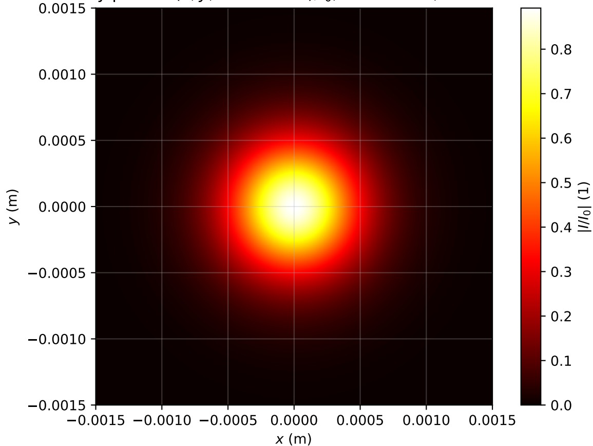
Intensity profile I(x, y, z = 1.751m)/I_0 , \text{Pin}=0.5\text{Pcr} , artificial time
